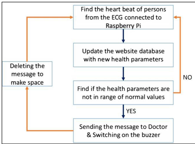
FIG3.1: CODING ALGORITHM FOR HEALTH CARE SYSTEM
