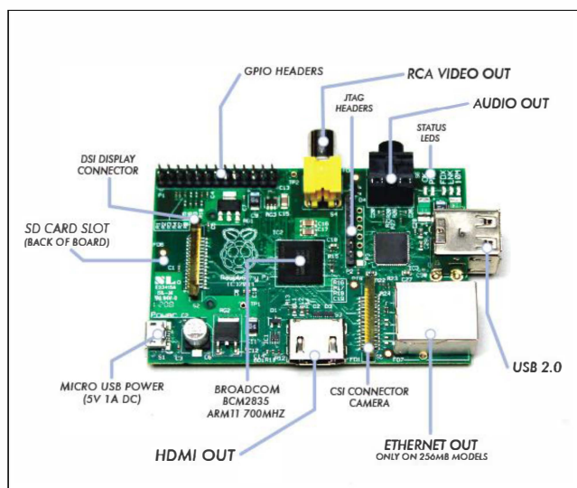
FIG1.1: RASPBERRY PI B+ BOARD
